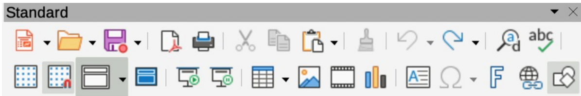
Figure 354: Standard toolbar
