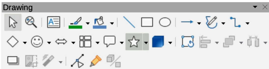
Figure 121: Drawing toolbar
