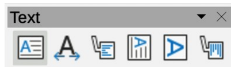
Figure 358: Text toolbar
