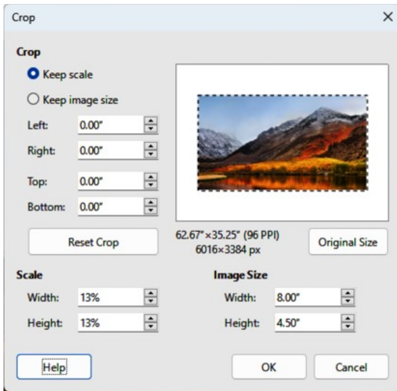
Figure 117: Crop dialog
