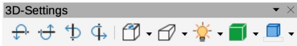
Figure 166: 3D-Settings toolbar
