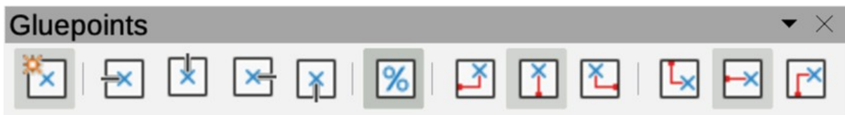
Figure 136: Gluepoints toolbar
