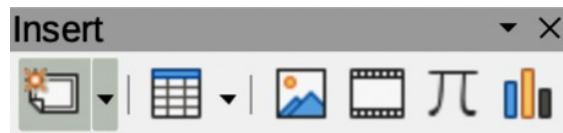
Figure 343: Insert toolbar
