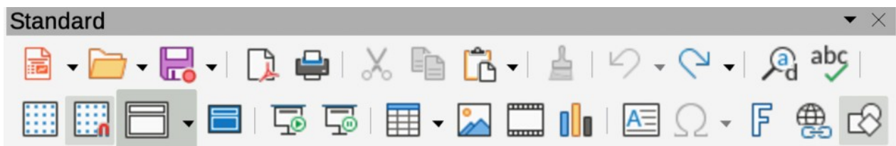
Figure 11: Standard toolbar
