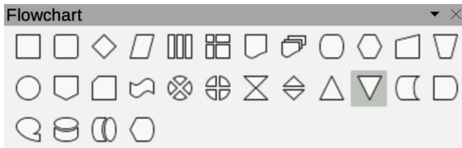
Figure 372: Flowchart subtoolbar
