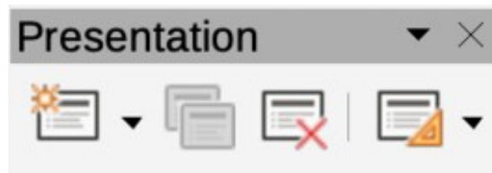
Figure 22: Presentation toolbar
