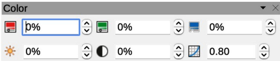
Figure 111: Color subtoolbar
