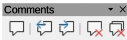
Figure 332: Comments toolbar
