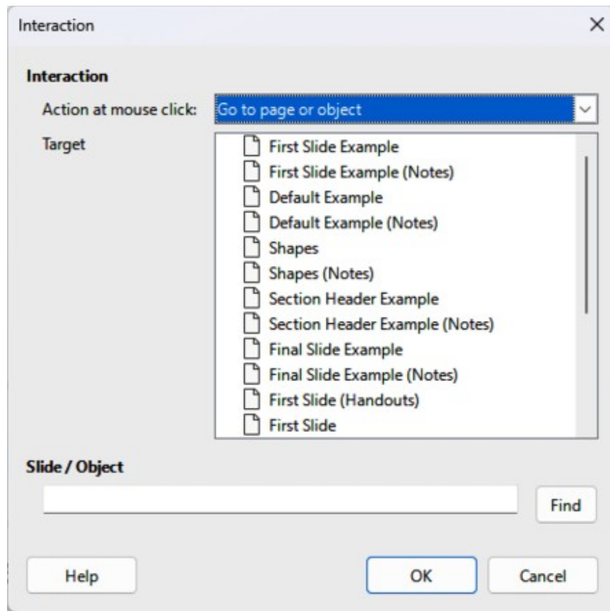
Figure 167: Interaction dialog
