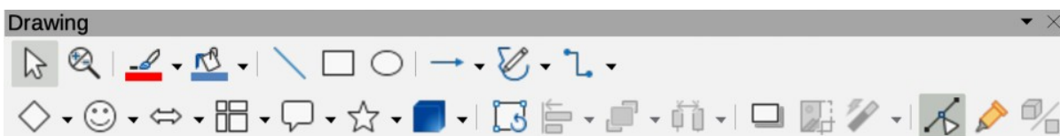
Figure 51: Drawing toolbar
