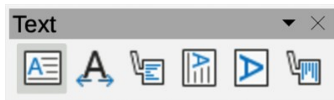
Figure 81: Text toolbar
