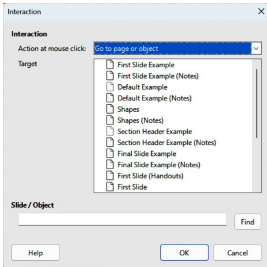
Figure 270: Interaction dialog
