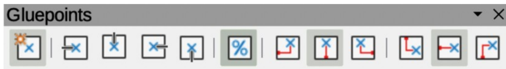
Figure 341: Gluepoints toolbar
