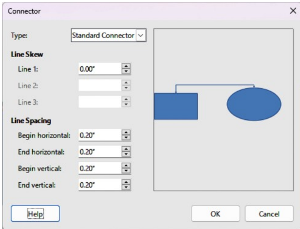
Figure 163: Connector dialog
