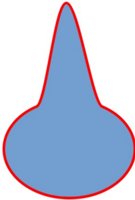
Figure 185: Example arrowhead
