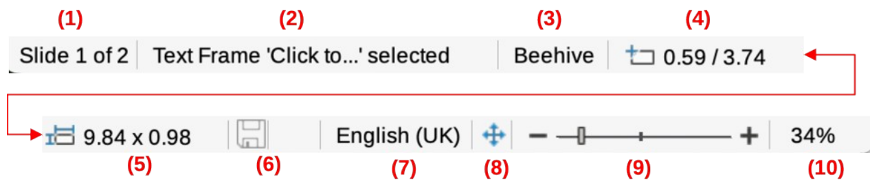
Figure 9: Status Bar
