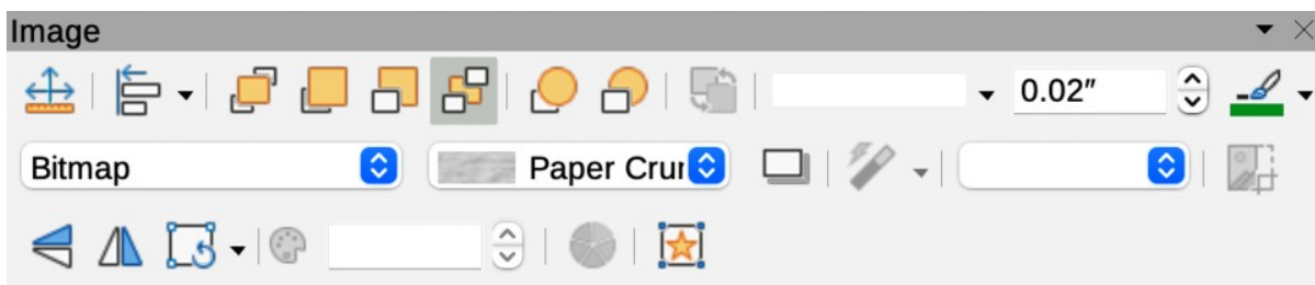
Figure 342: Image toolbar
