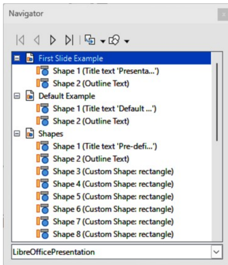
Figure 10: Navigator dialog
