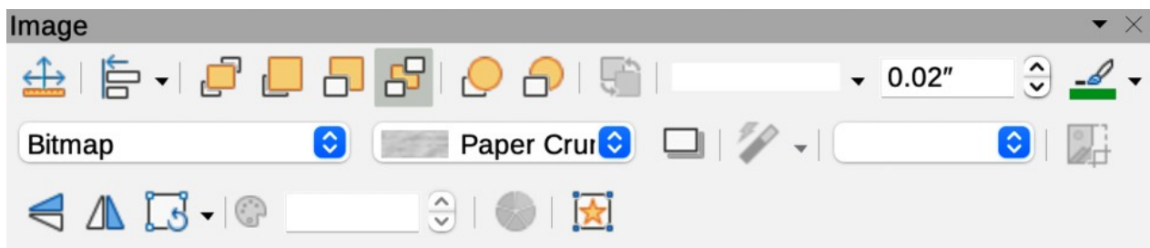
Figure 107: Image toolbar
