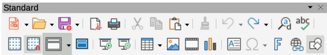
Figure 283: Standard toolbar
