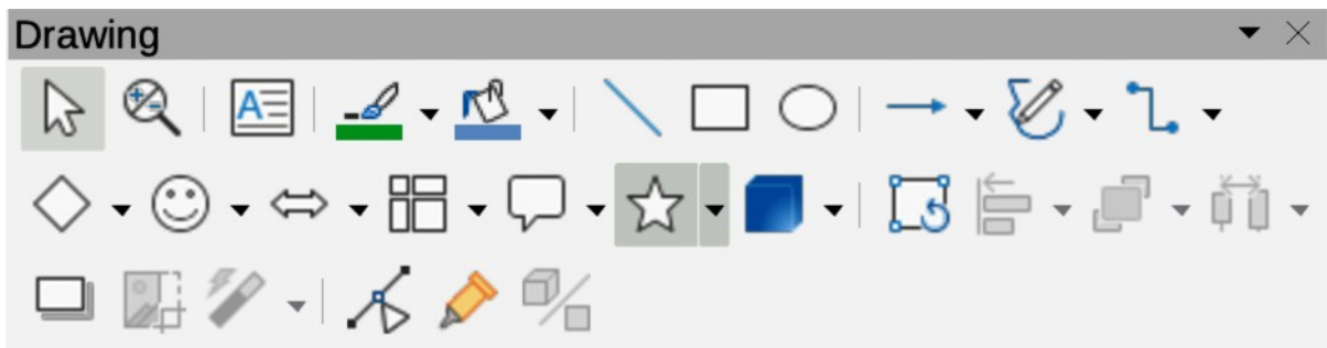
Figure 334: Drawing toolbar
