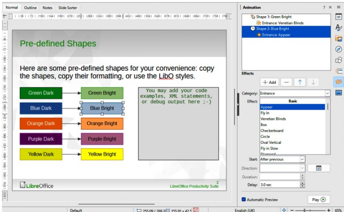
Figure 269: Example animation
