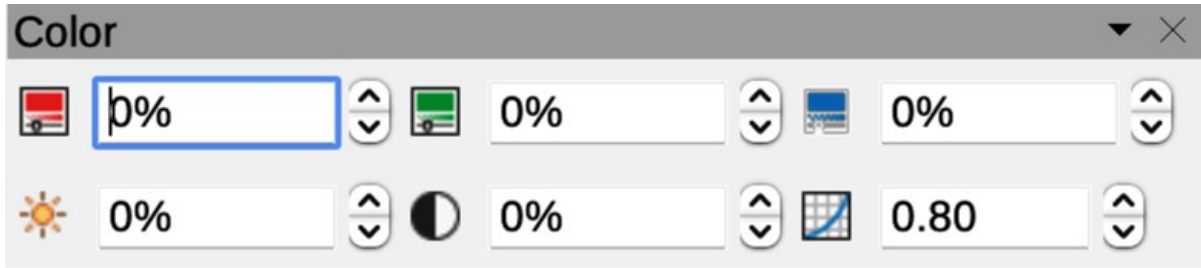
Figure 368: Color subtoolbar
