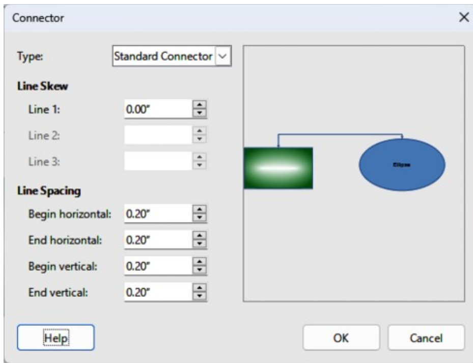
Figure 206: Connector dialog
