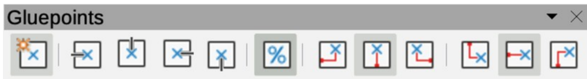
Figure 164: Gluepoints toolbar
