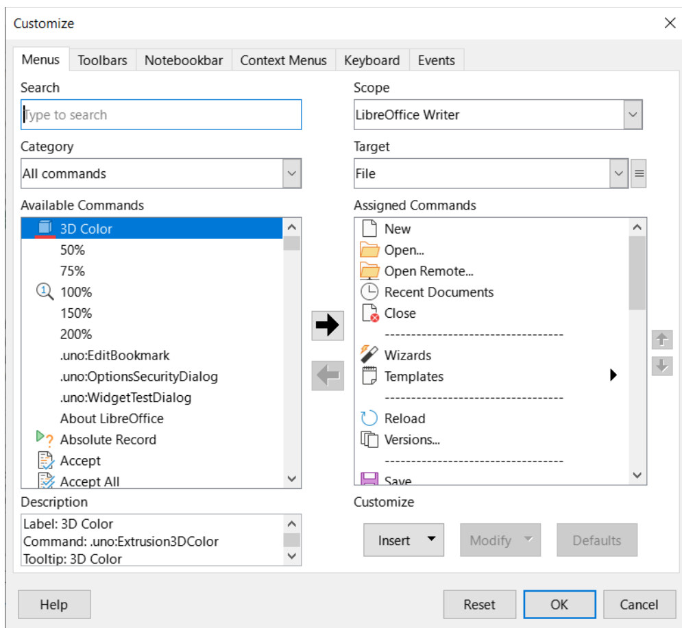
Figure 396: Customize dialog — Menus page
