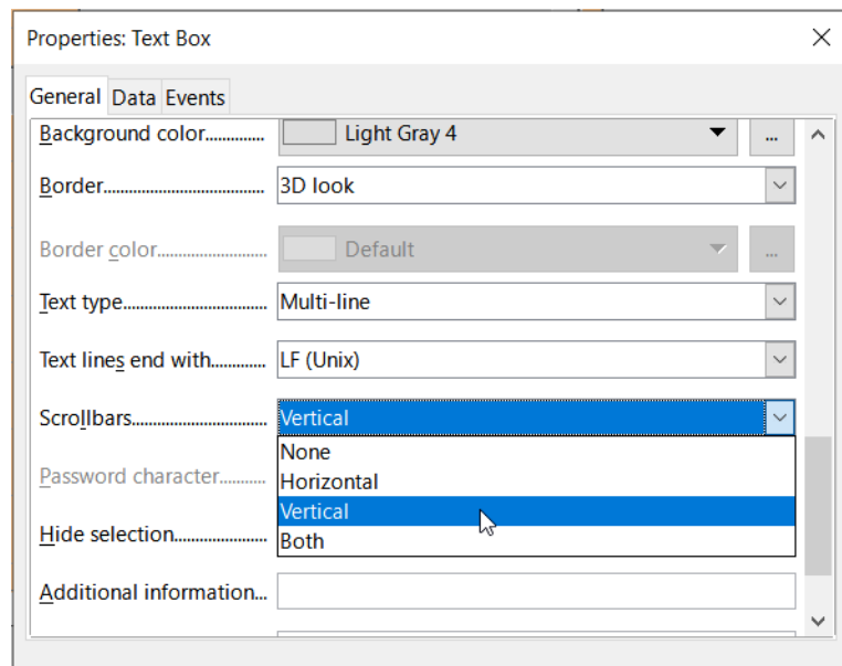
Figure 271: Scroll bar selections in the Properties dialog
