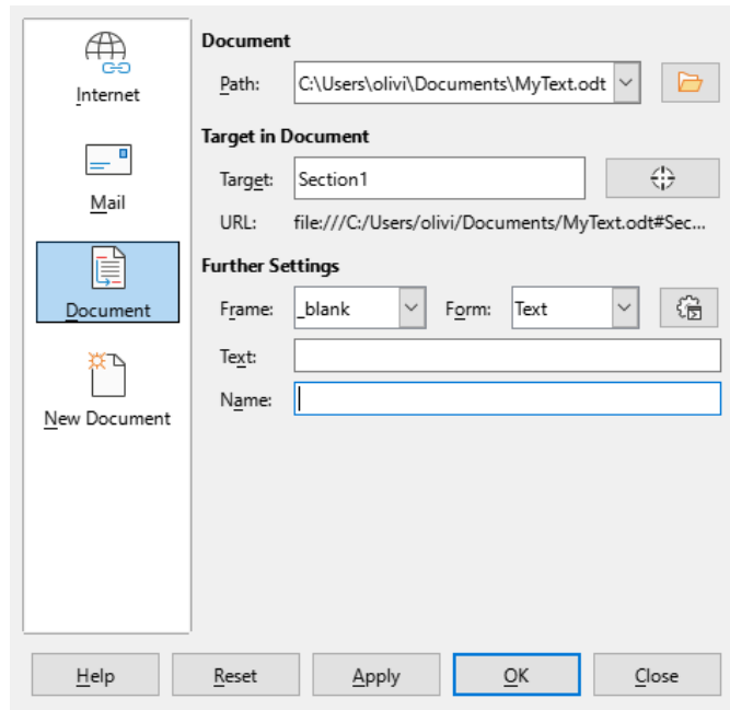
Figure 111: Hyperlink dialog — Document page
