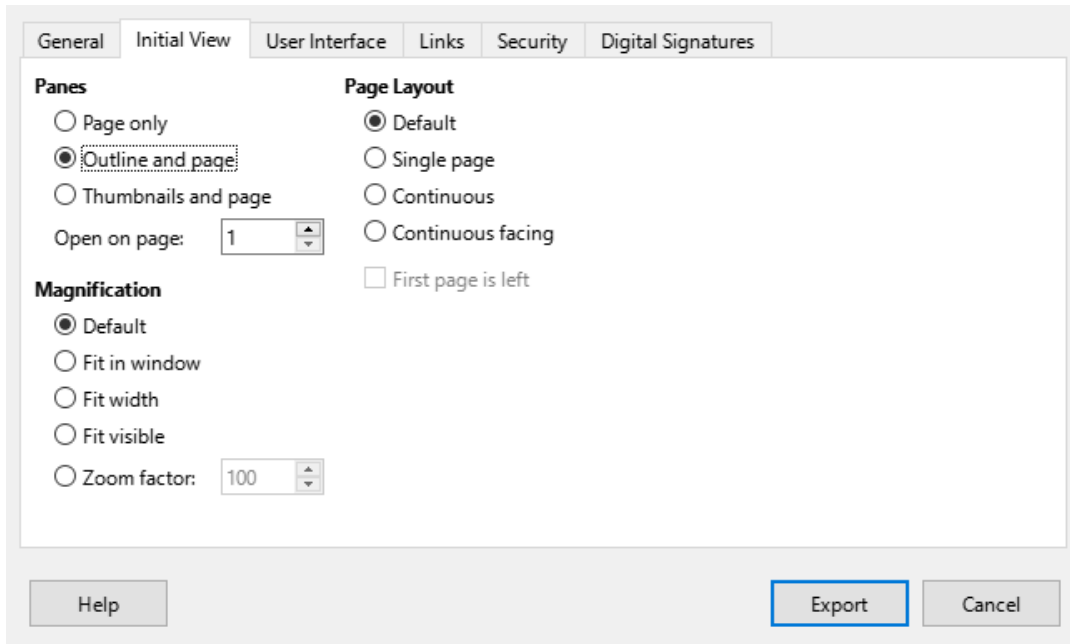
Figure 320: PDF Options dialog — Initial View page
