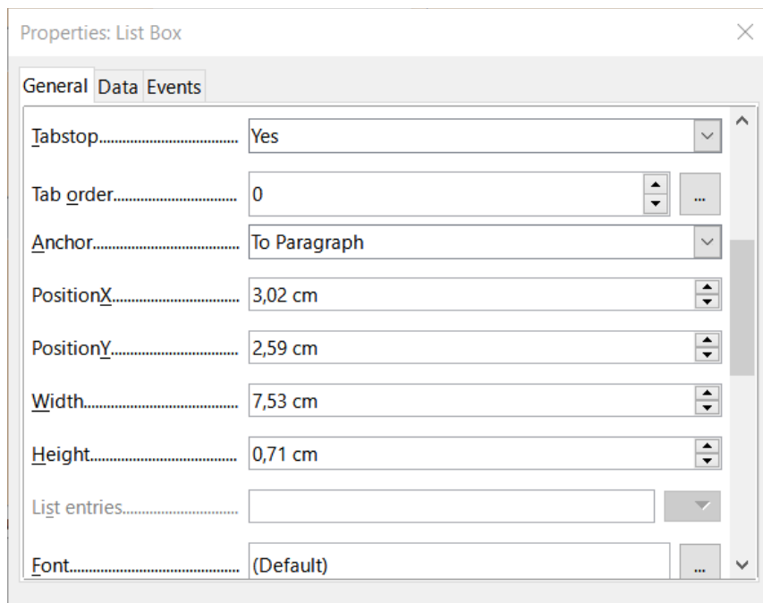
Figure 268: Modifying listbox properties
