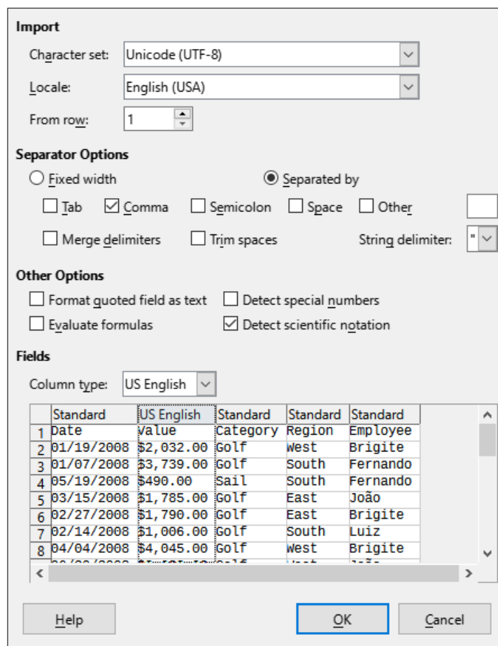
Figure 56: Text Import dialog
