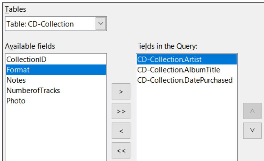
Figure 293: First page of the Query Wizard
